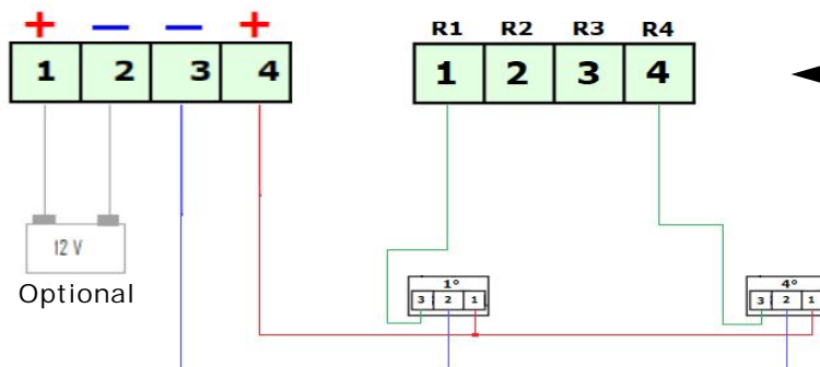
Connection of probes and eventual battery
