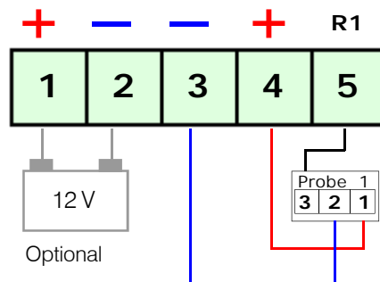
Connection of probes and eventual battery
