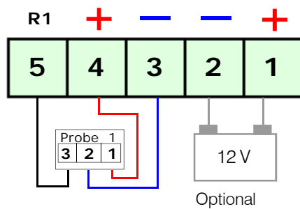
Connection of probes and eventual battery
